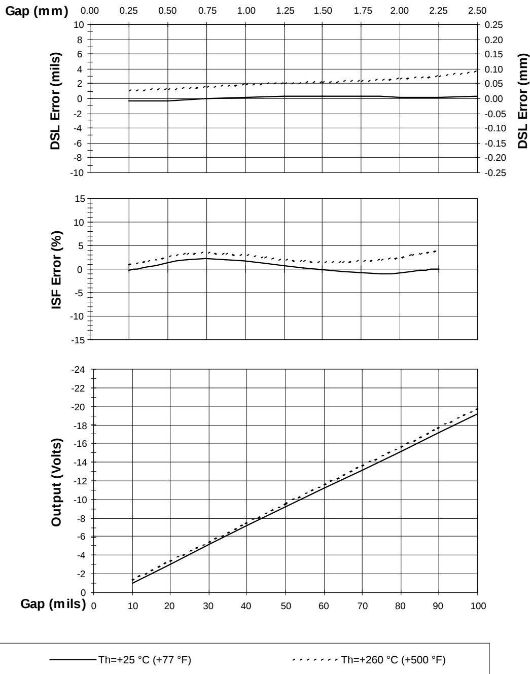
Figure 9: Typical 3300 XL Extended Temperature Range Probe and 8m Extended Temperature Range Extension Cable at T_h (Proximitior Sensor and Probe Tip with 1-foot Cable are at +25 °C)
